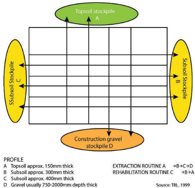
Figure B.10.5: Procedure for removal of overburden and stockpiling
