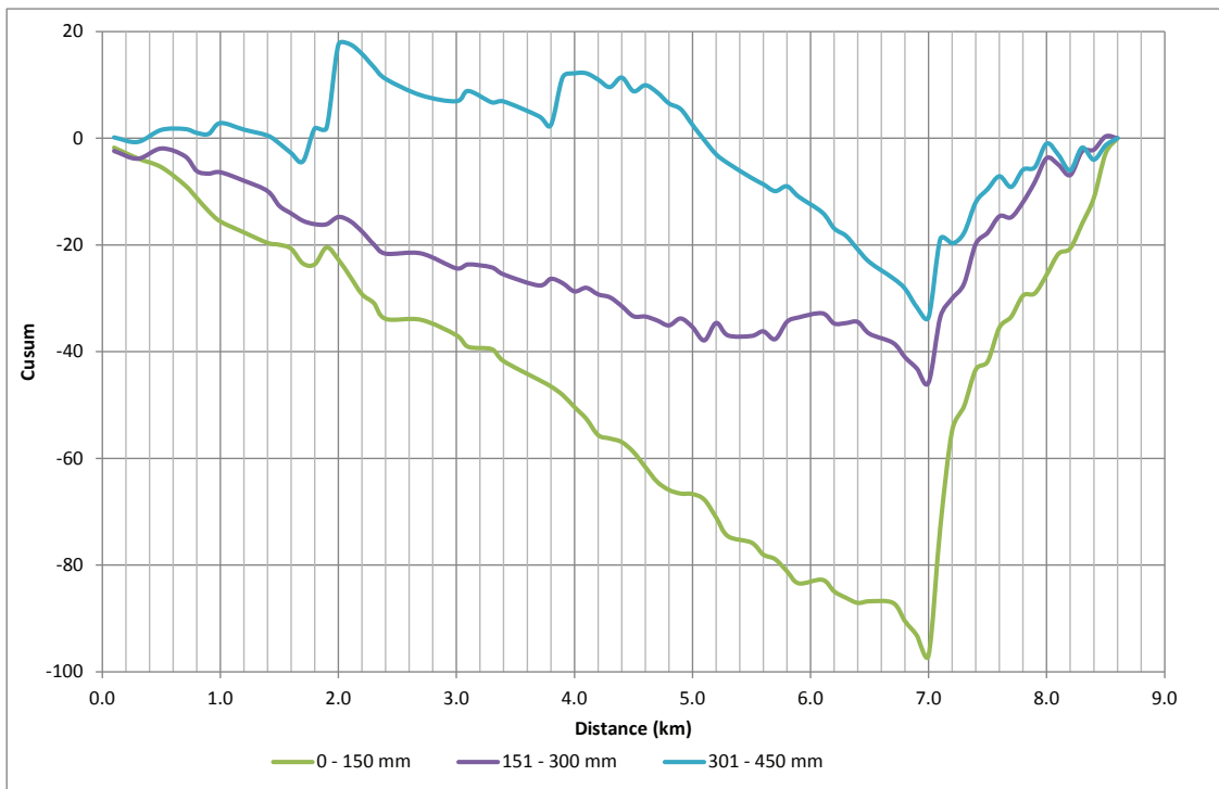
Figure 5: CUSUM versus distance for the DN_{150} , DN_{151-300} and DN_{301-450} results
