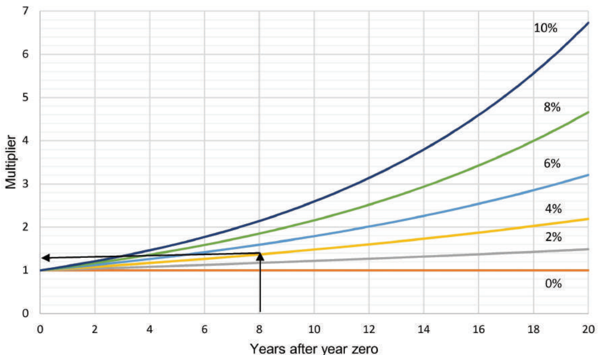
Figure B.2.5: Multiplier to obtain AADT in any year for different growth rates
