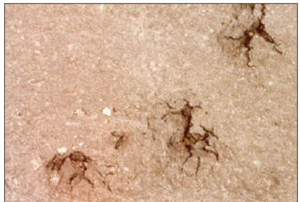
Figure B.4.16: Salt damage as 'blistering', 'heaving' & 'fluffing' of the wearing course.
