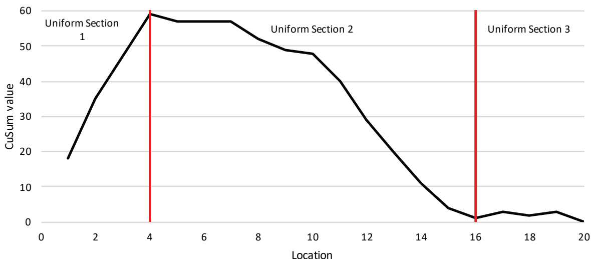
Figure B.4.2: Example of a Cumulative Sum Plot
