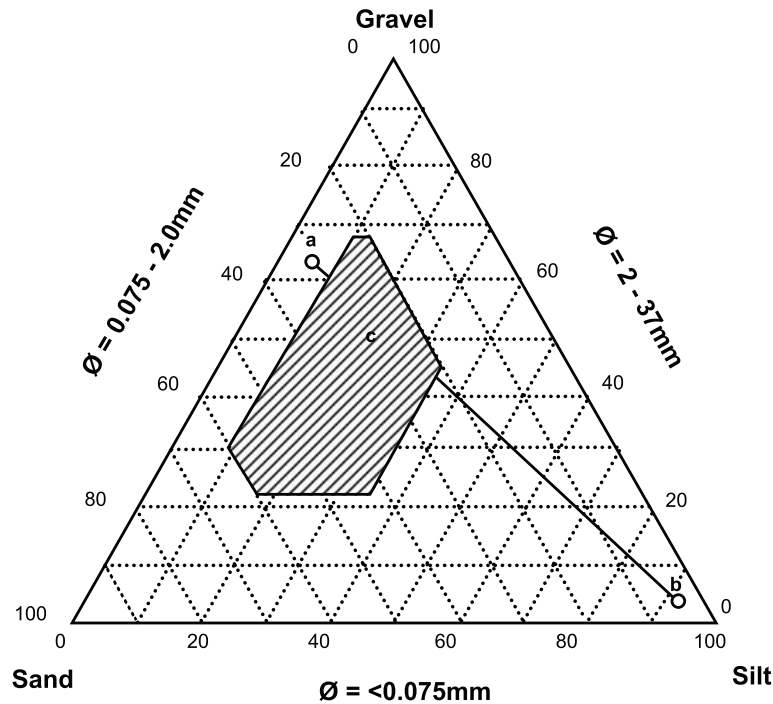
Figure B.5.5: Ternary diagram for determining proportions for blending of materials
