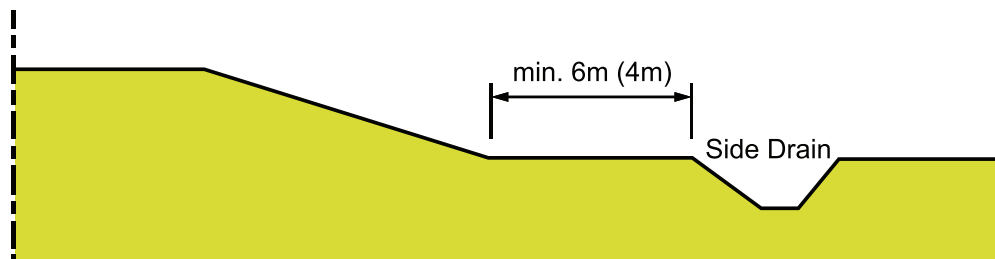
Figure B.4.8: Location of side drains in expansive soils
