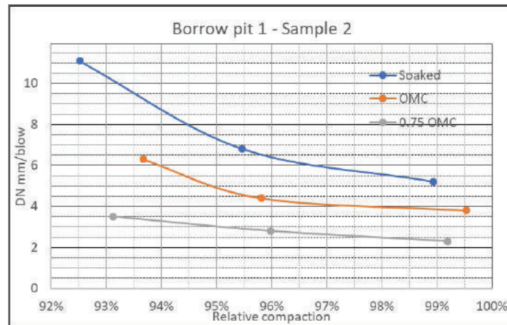
Figure 3: DN/density/moisture
