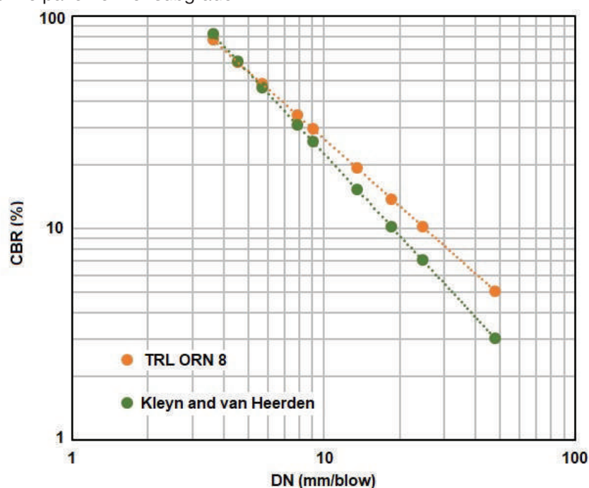
Figure B.4.1: Correlation between DN and CBR
