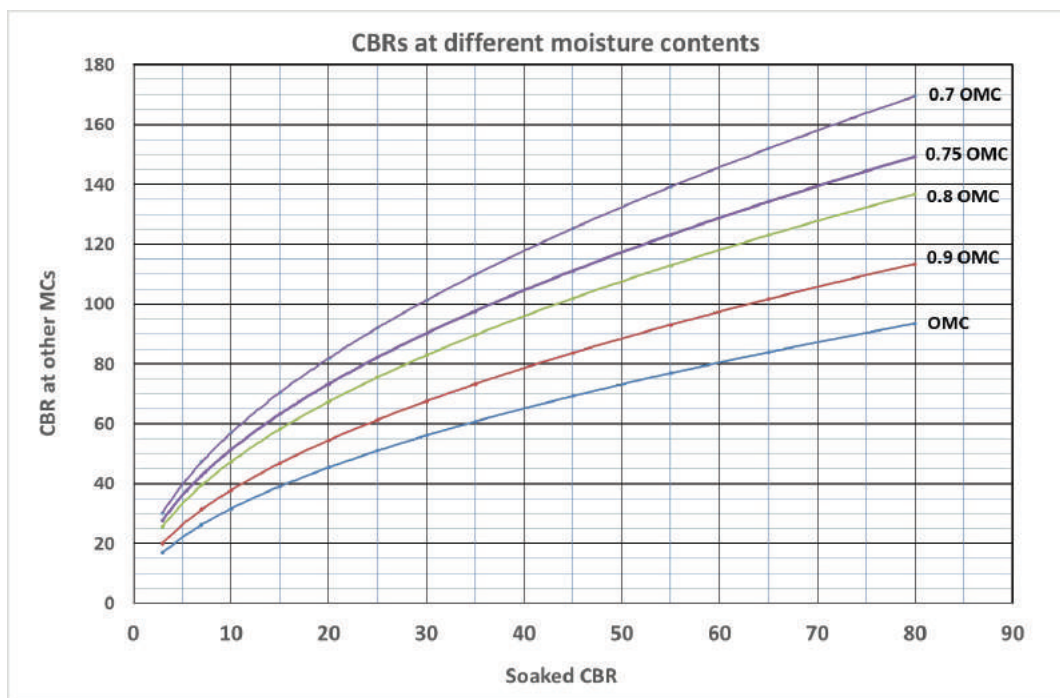
Figure 2: CBRs at different moisture contents
