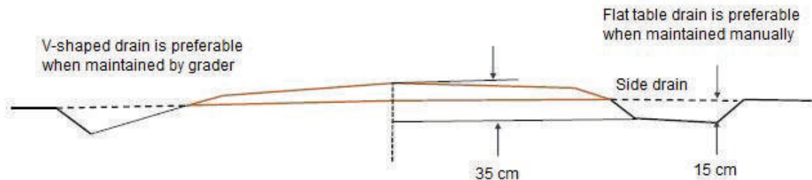
Figure B.7.1: Cross-section of partially engineered earth road
