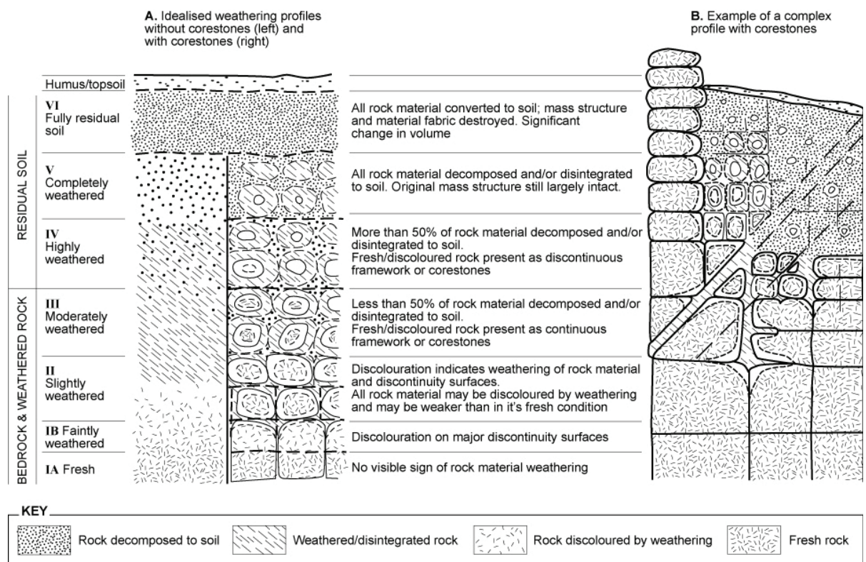
Figure 1: Weathering grade classification
