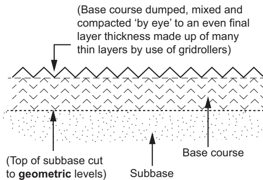
Figure B.9.13: Procedure to finish off natural gravel base course
