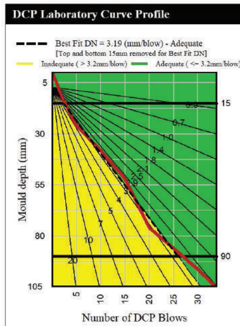
Figure 2: Typical output from the Laboratory DN test
