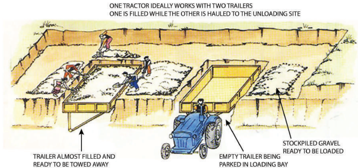
Figure B.10.9: Borrow pit arrangement using labor-based methods
