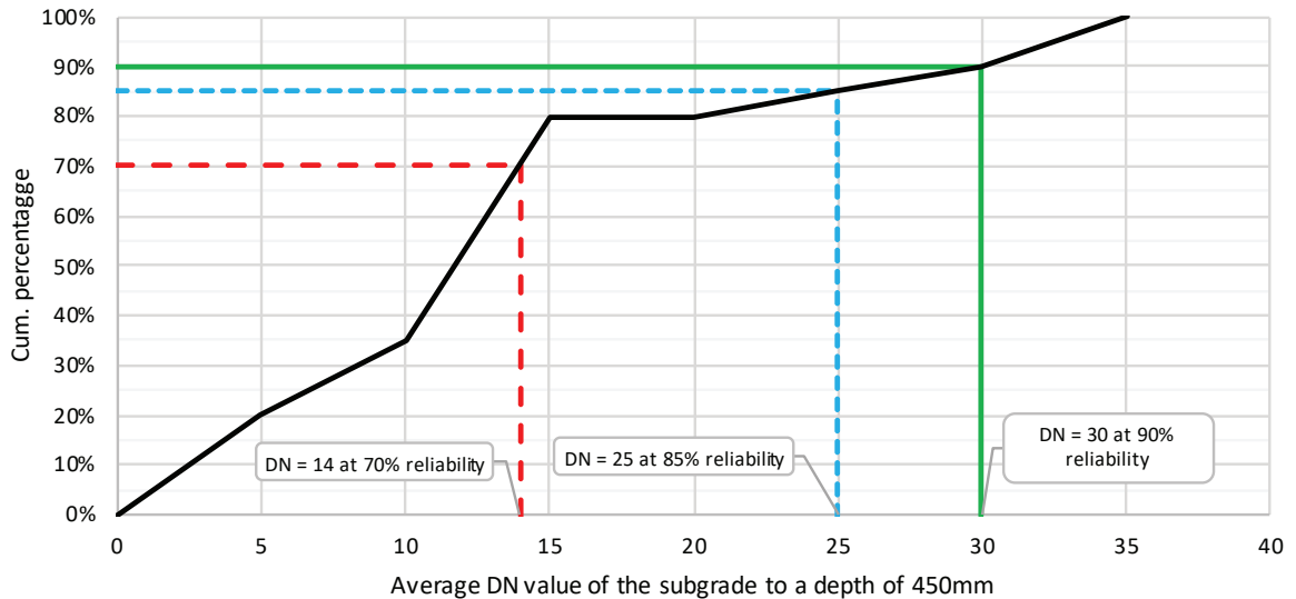
Figure B.4.3: Example of cumulative distribution plot
