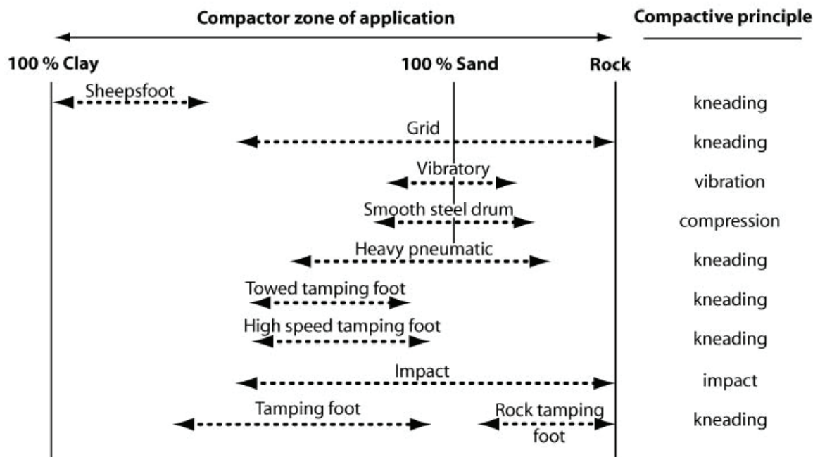
Figure B.9.9: Compaction Equipment Guide
