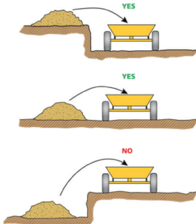
Figure B.10.8: Trailer loading height
