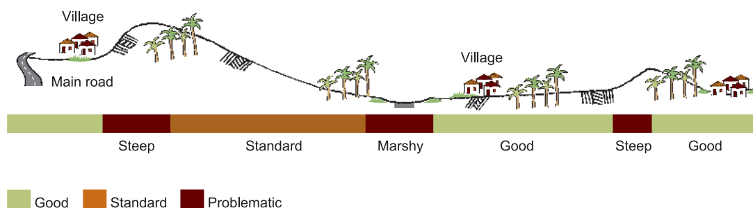
Figure B.1.9: Environmentally Optimized and Spot Improvement Design
