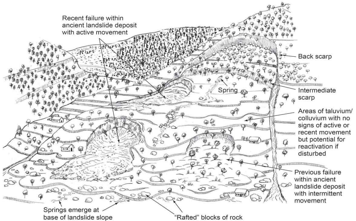
Figure B.3.1: Features commonly observed in landslide areas
