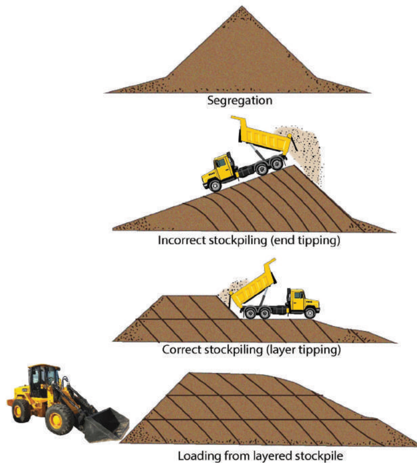
Figure B.10.11: Correct stockpiling to avoid segregation
