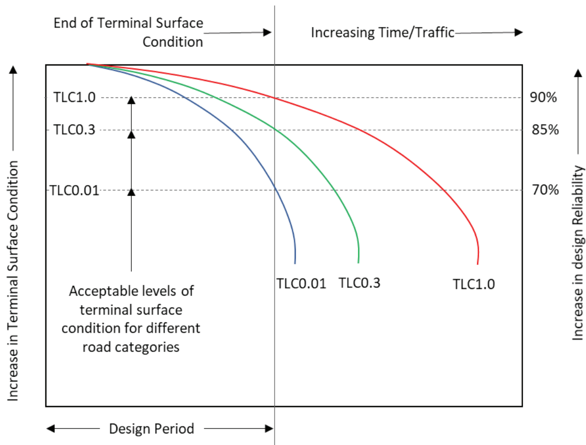
Figure B.1.6: Design reliability in relation to road category and terminal surface condition
