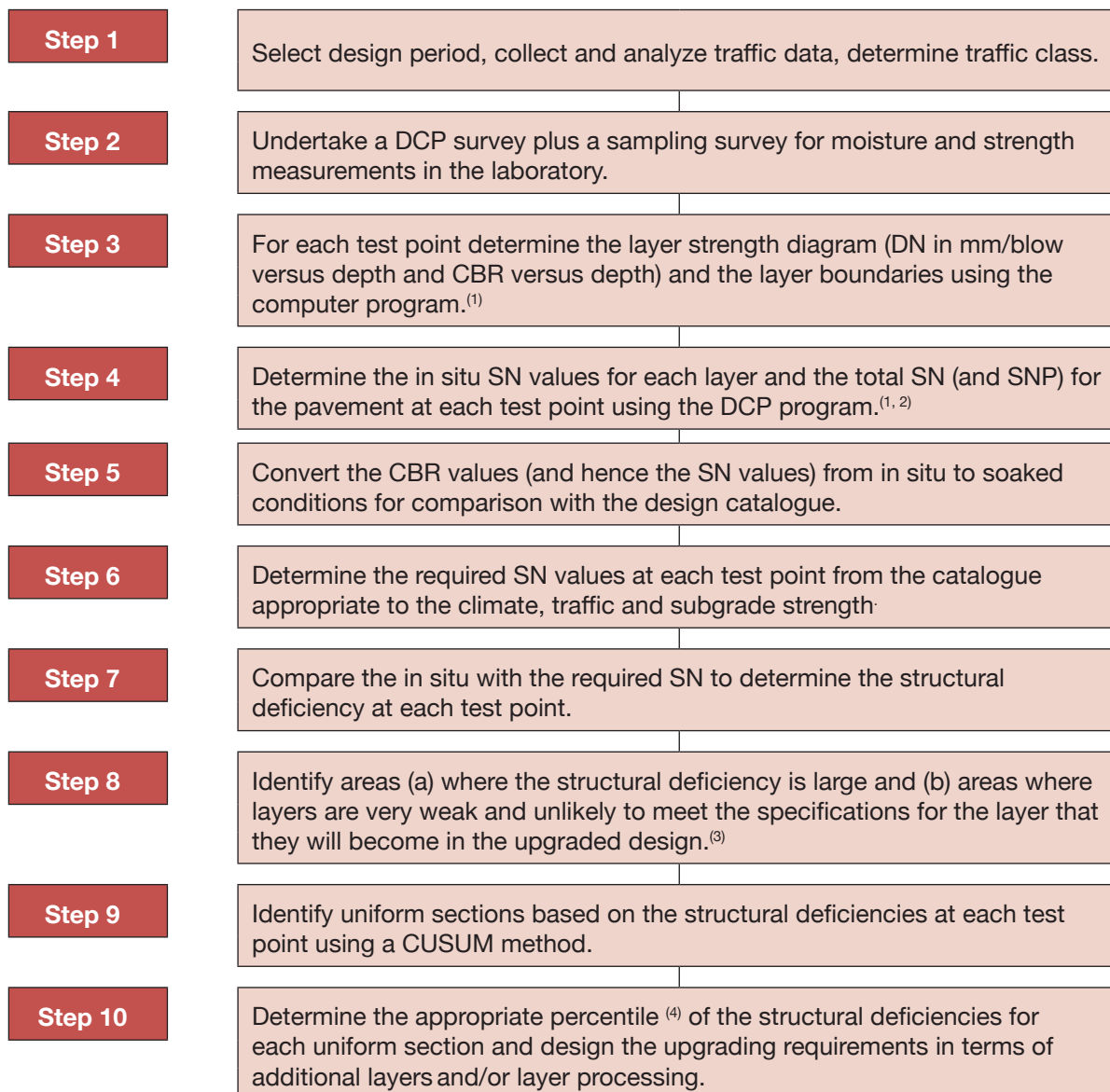
Figure 1: DCP-CBR method - Flow diagram for upgrading an existing road
