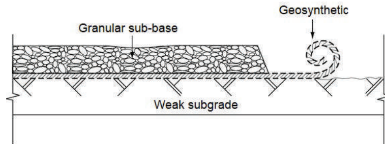
Figure B.4.18: Use of geosynthetic to separate a sub-base from the subgrade
