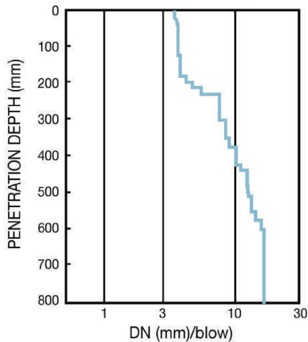
Figure B.6.4: Typical DN with depth profile
