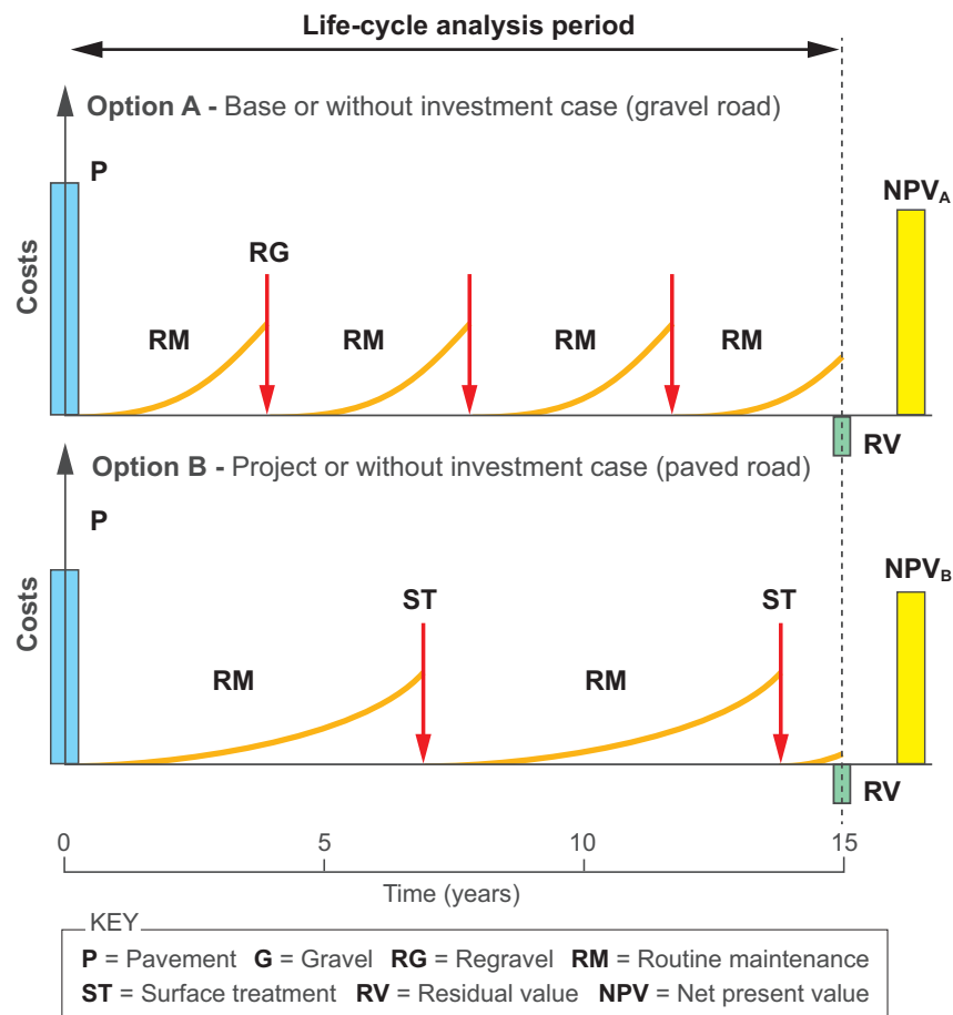
Figure B.8.8: Typical components of an LCC: gravel versus paved road
