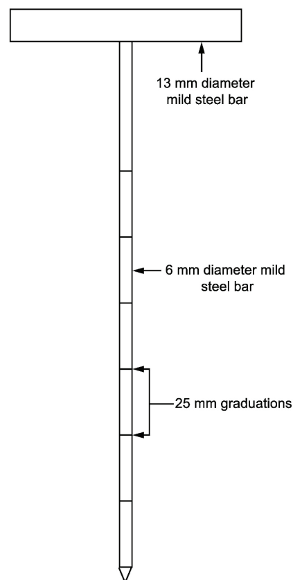
Figure B.11.3: Probe for assessing layer thickness
