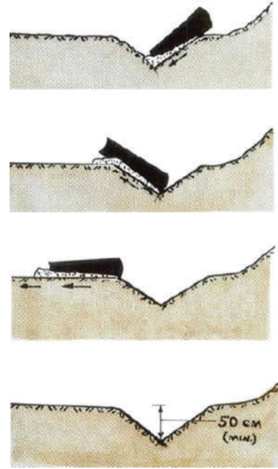
Procedure for cleaning a side drain
