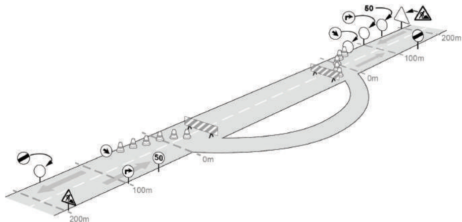
Figure E.6.1: Sign posting for diversion of traffic off the road
