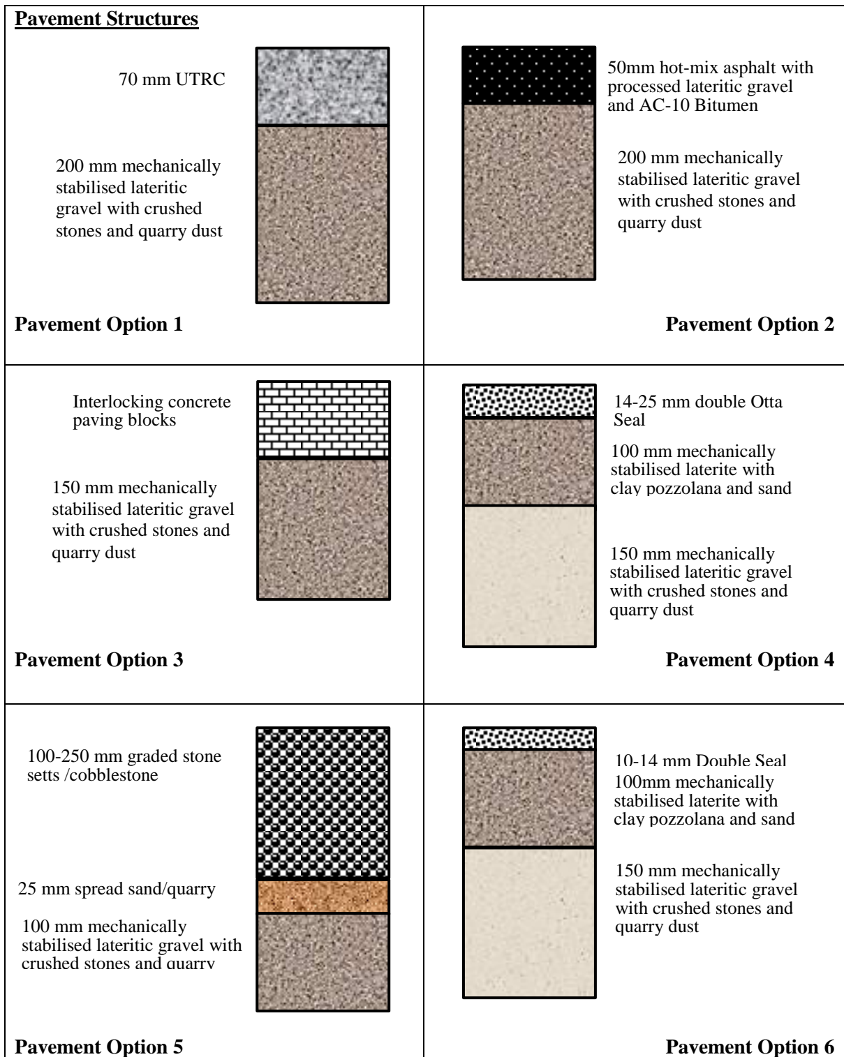
Figure 3: Cross Sections of Proposed Structures for Different Surfacing Options
