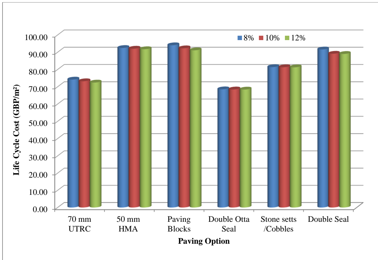
Figure 4: Comparison of life-cycle cost at three discount rates
