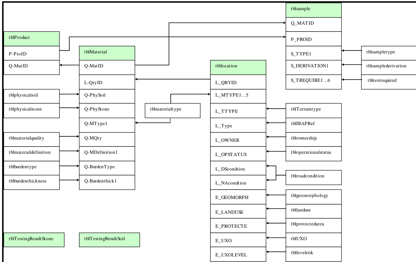
Figure B1 Database Table and Field Relationship
