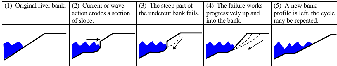
Figure 1. Diagrammatic Representation of the Erosion-Mass Failure Combination Governing Bank Erosion
