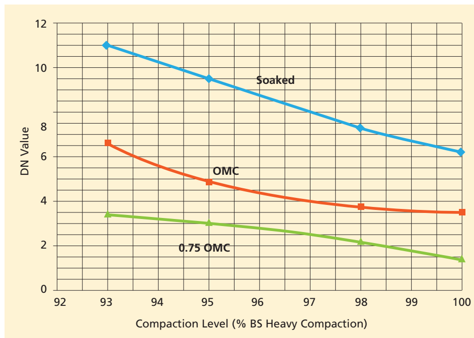
Figure 7-7: DN/density/moisture relationship
