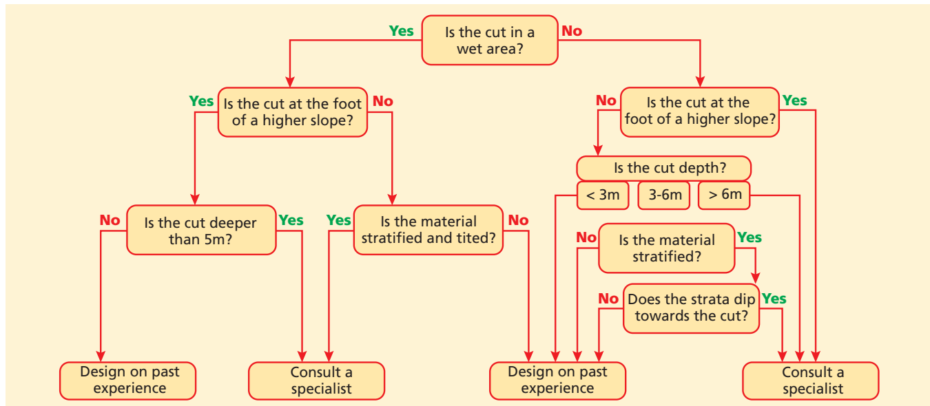
Figure 6-12: Decision chart for design of road cuttings
