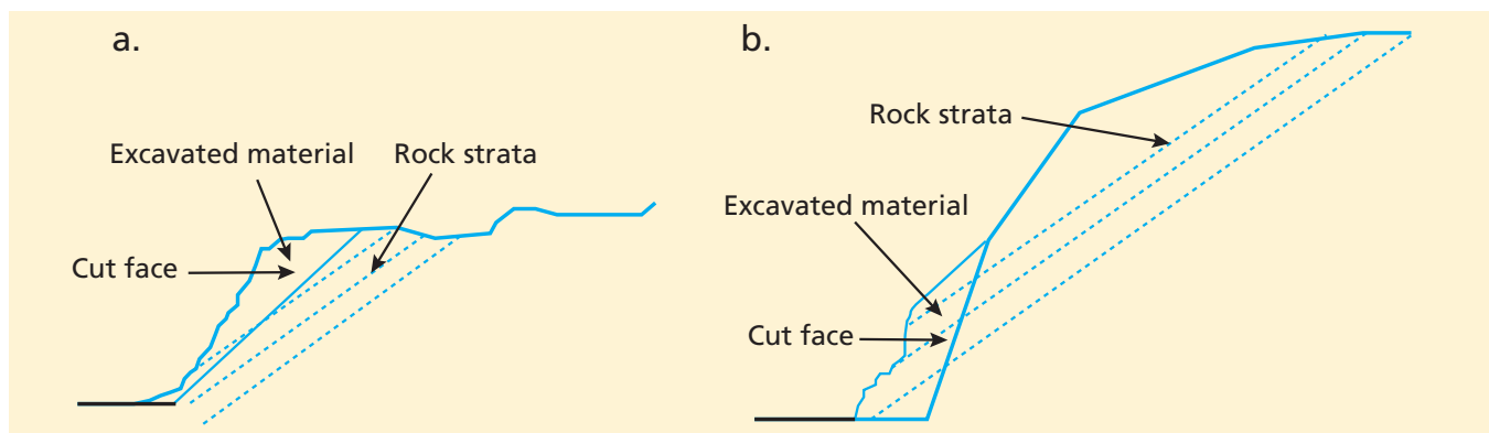
Figure 6-13: Effect of topography on volume of failed material
