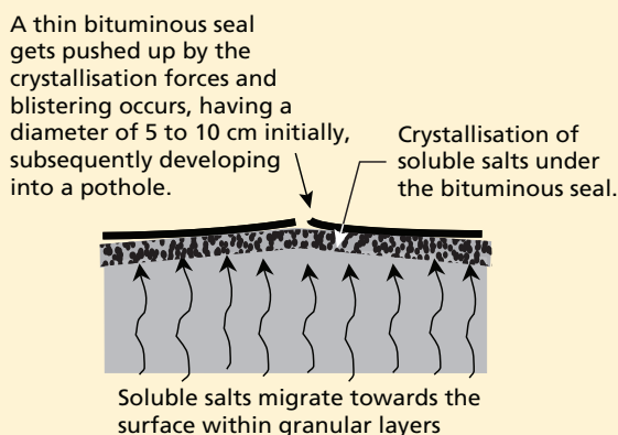
Figure 6-9: Mechanism of soluble salt damage to bituminous surfacings
