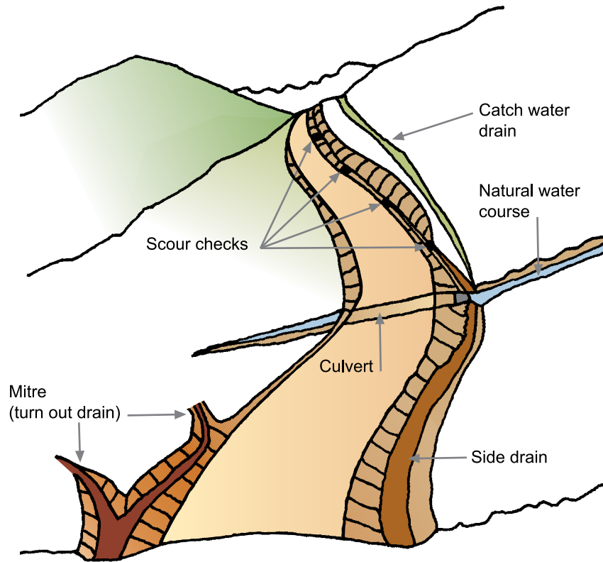
Figure 2-3: Drainage elements
