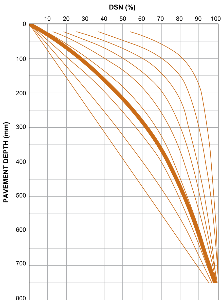
Figure 5A-4: Balanced structure
