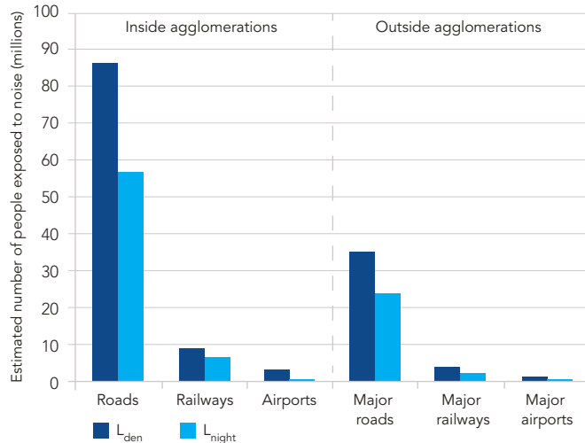
FIGURE 5.4: Exposure to Unhealthy Traffic Noise in EU Member States (Excluding Croatia) in 2012
